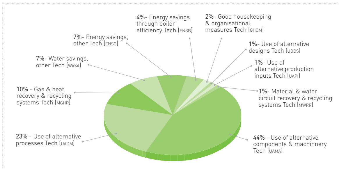
GRAPH II.4 - REDUCTION OF ENERGY CONSUMPTION: MAIN TECHNIQUES
