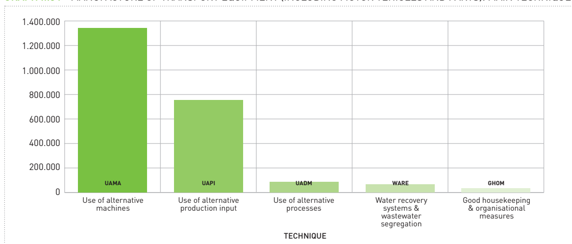
GRAPH II.54 - MANUFACTURE OF TRANSPORT EQUIPMENT (INCLUDING MOTOR VEHICLES AND PARTS): MAIN TECHNIQUE
